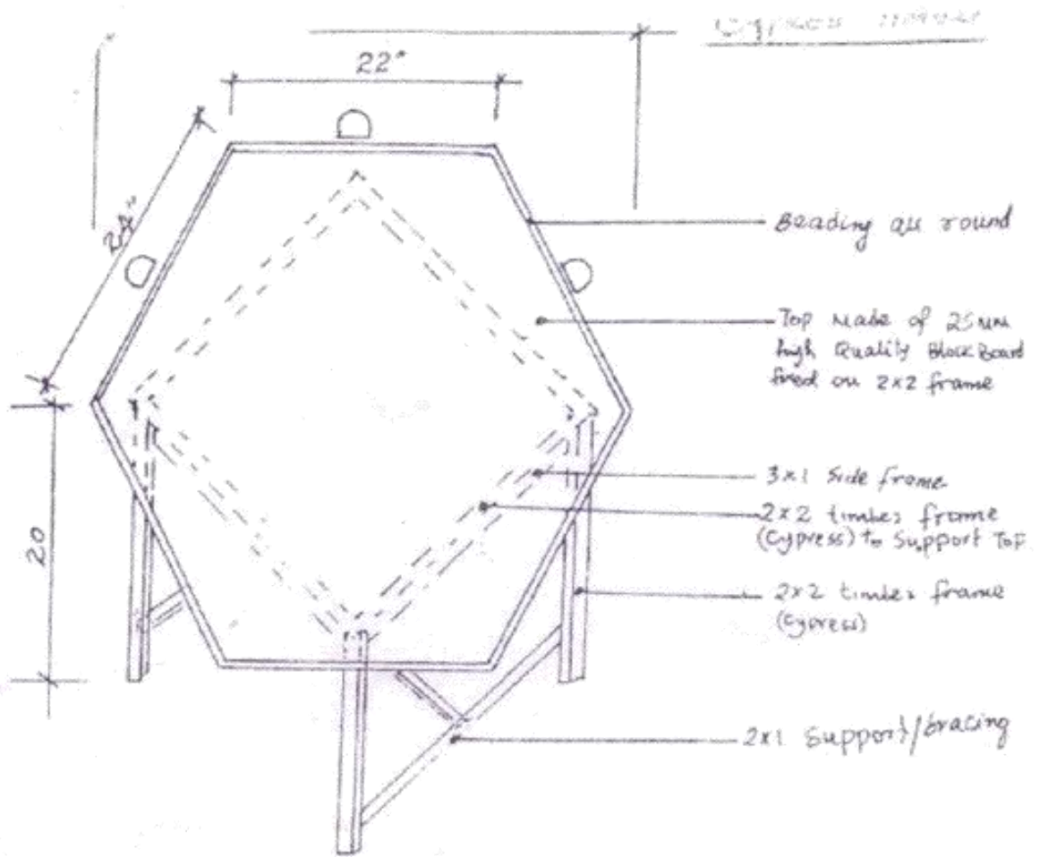
DEE-SHODU TABLE AND CHAIR
